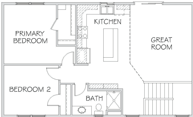
MAIN LEVEL
