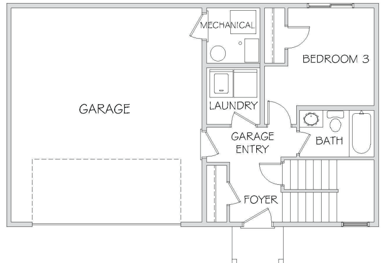
UPPER LEVEL
