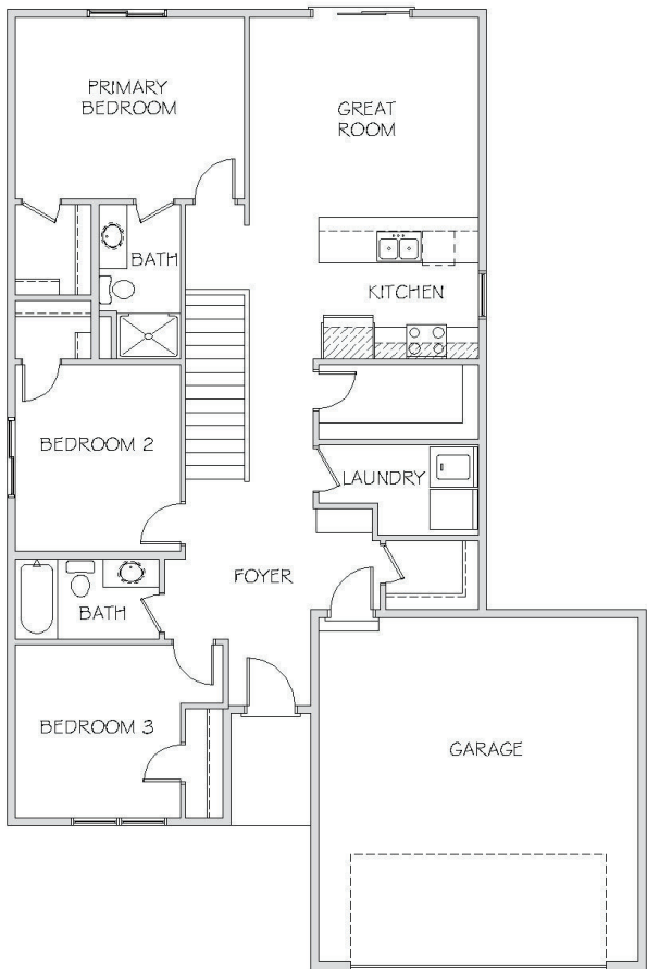
MAIN LEVEL
