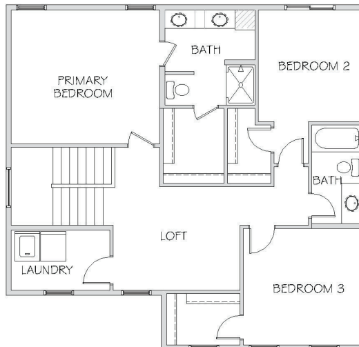
UPPER LEVEL
