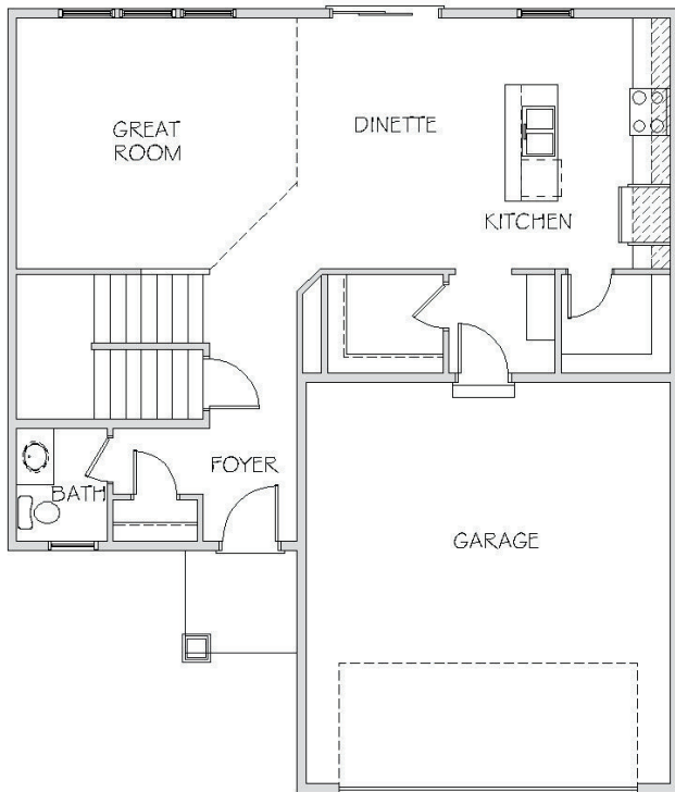
MAIN LEVEL
