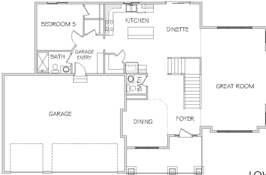
LOWER LEVEL
