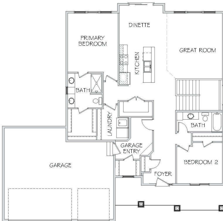
MAIN LEVEL
