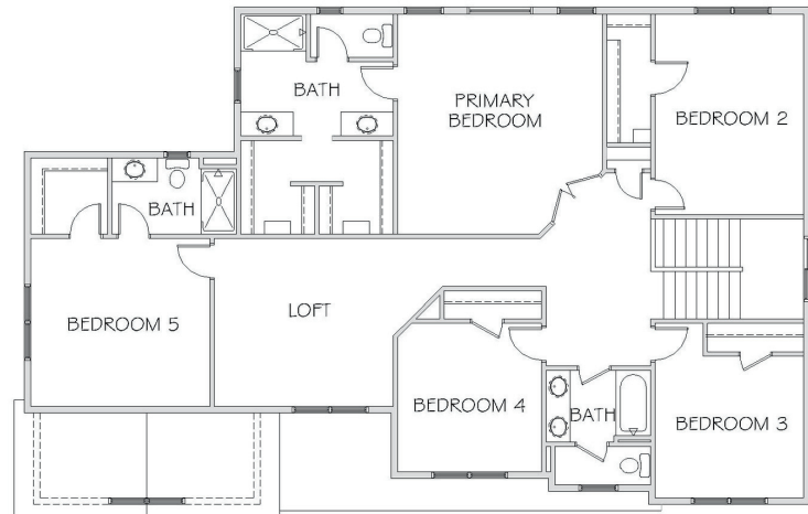
UPPER LEVEL
