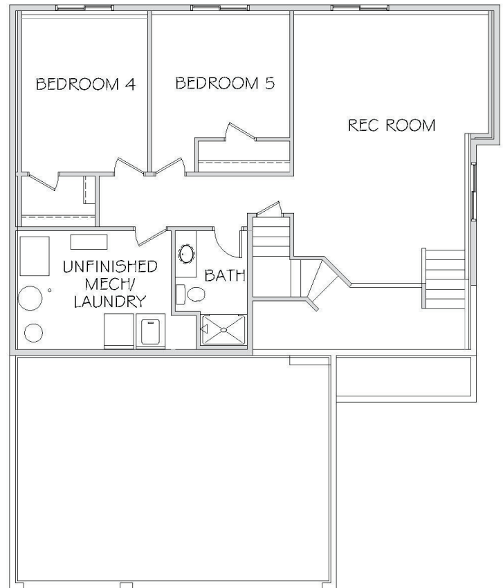
LOWER LEVEL
