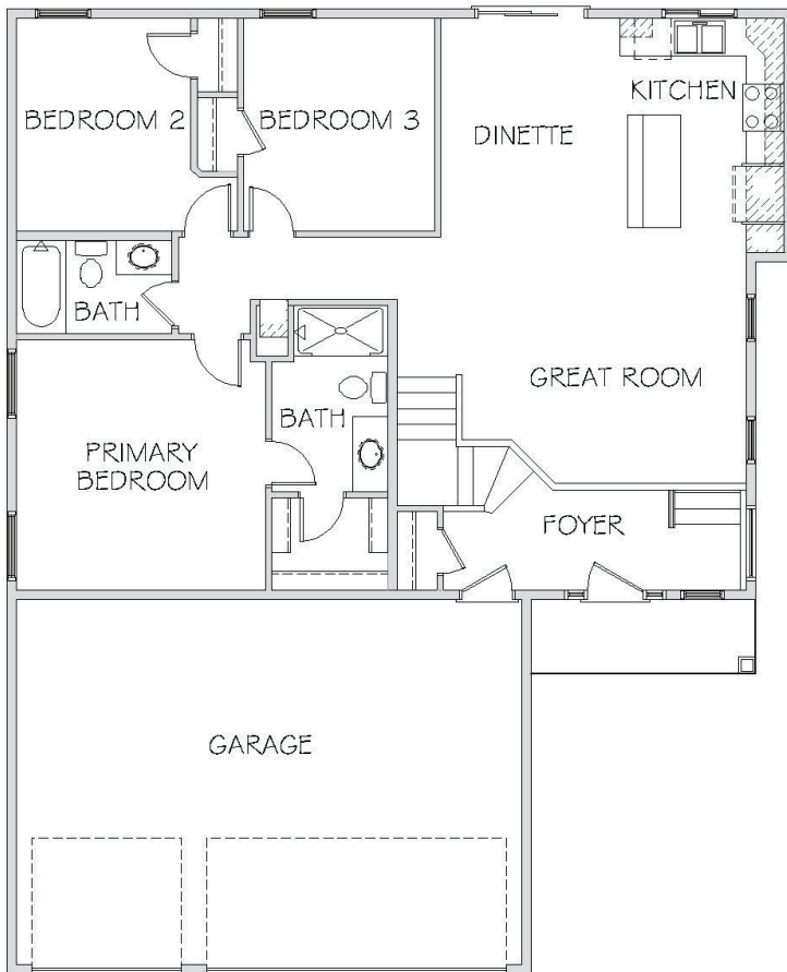
MAIN LEVEL
