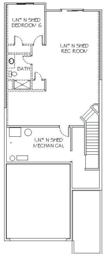
LOWER LEVEL
