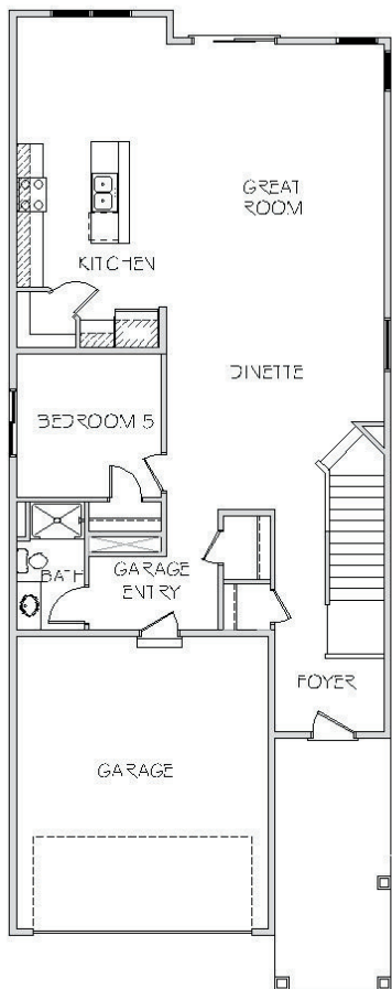
MAIN LEVEL
