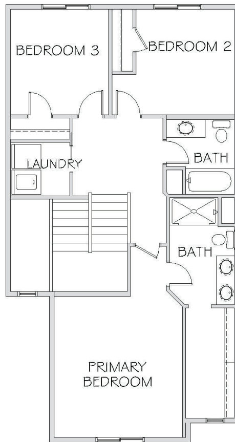
UPPER LEVEL
